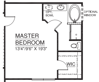
OPT. SEPARATE TUB AND SHOWER
